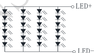
B/L CIRCUIT DIAGRAM
