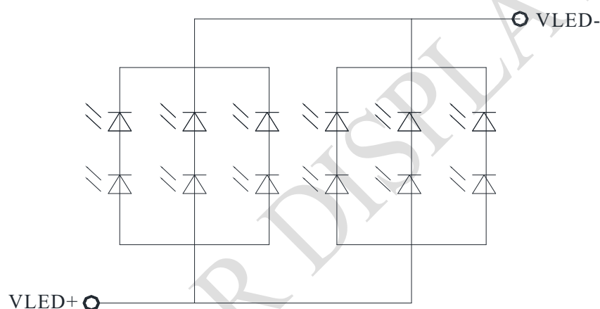
CIRCUIT DIAGRAM
