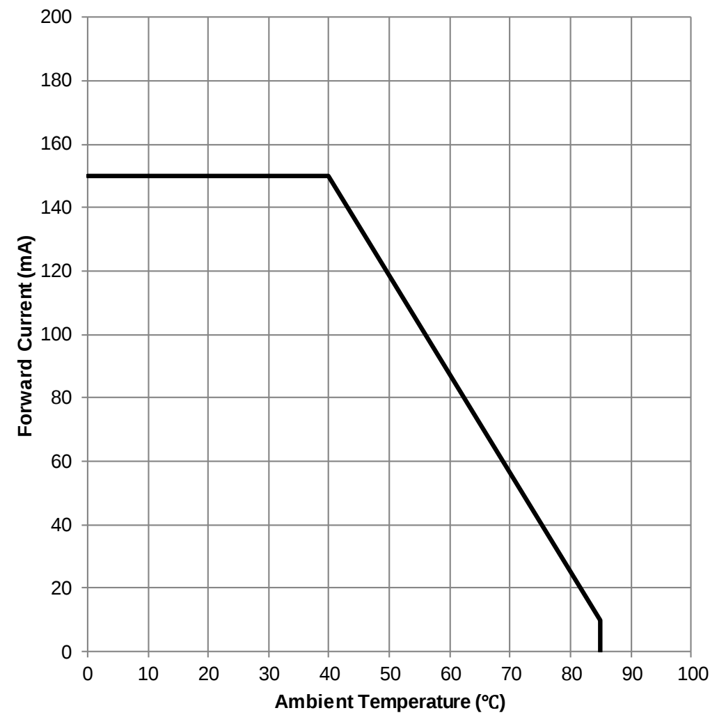
Derating Curve:
