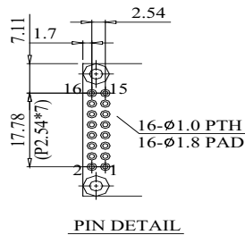
PIN DETAIL
