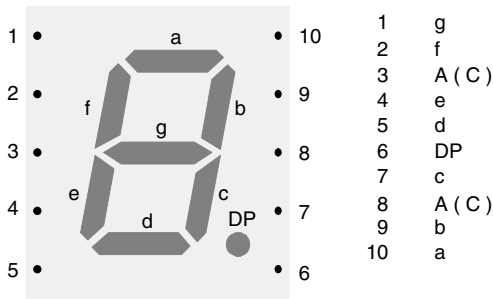
Fig. 13 - TDS.31..
