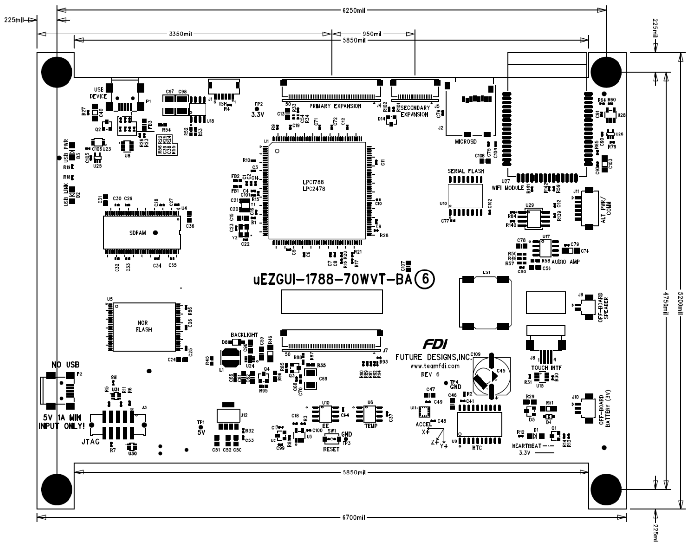
Figure 2 –UEZGUI-1788-70WVT Component View
