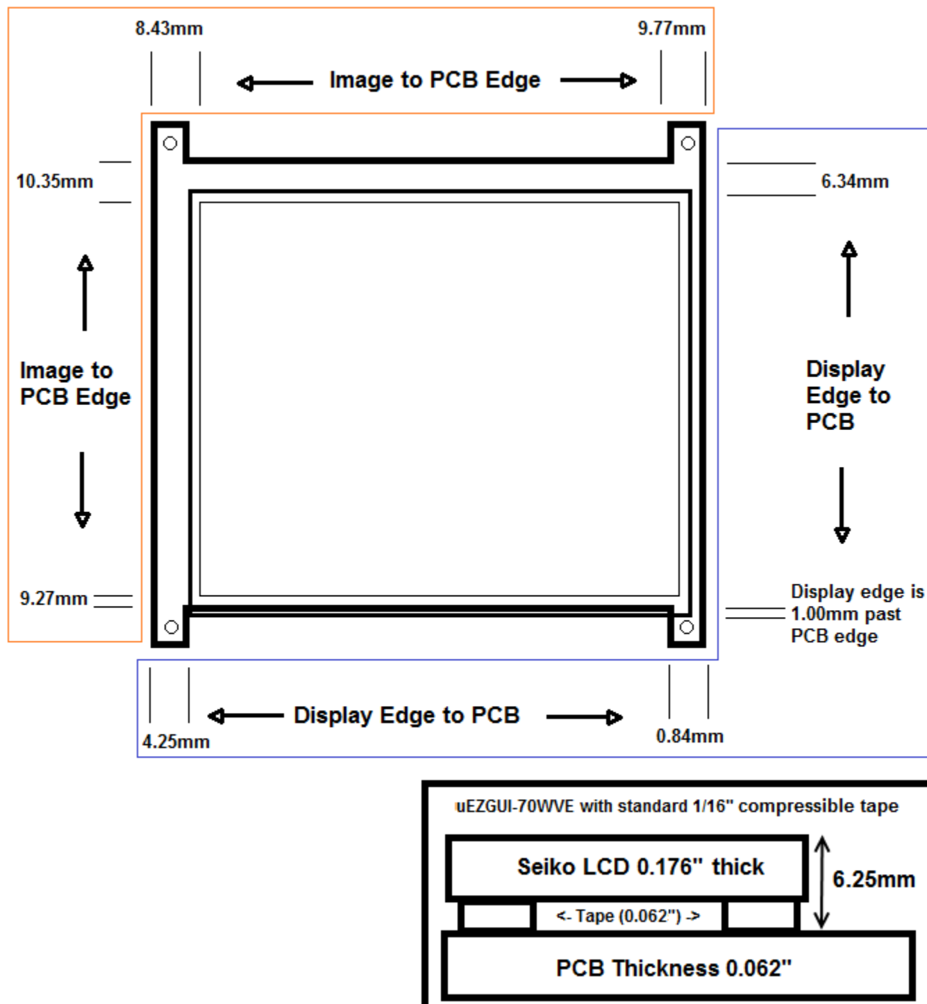
Figure 6 – UEZGUI-1788-70WVE Dimensions and Stack-up
