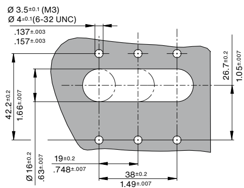
Cut-out dimensions recommended panel thickness 1 - 2.5 mm
