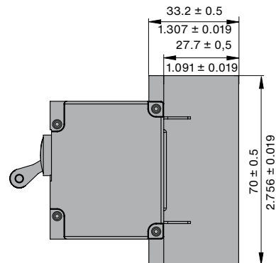
Approval variant L (UL489)
