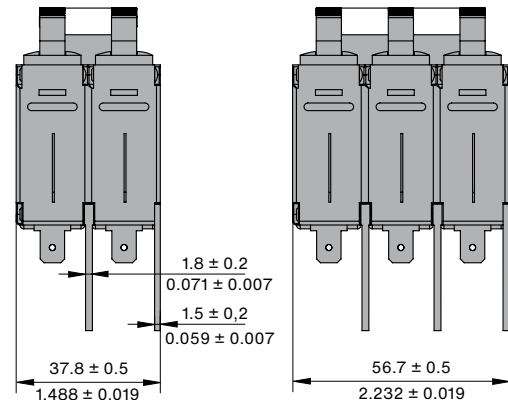
Cut-out dimensions recommended panel thickness 1 - 2.5 mm
