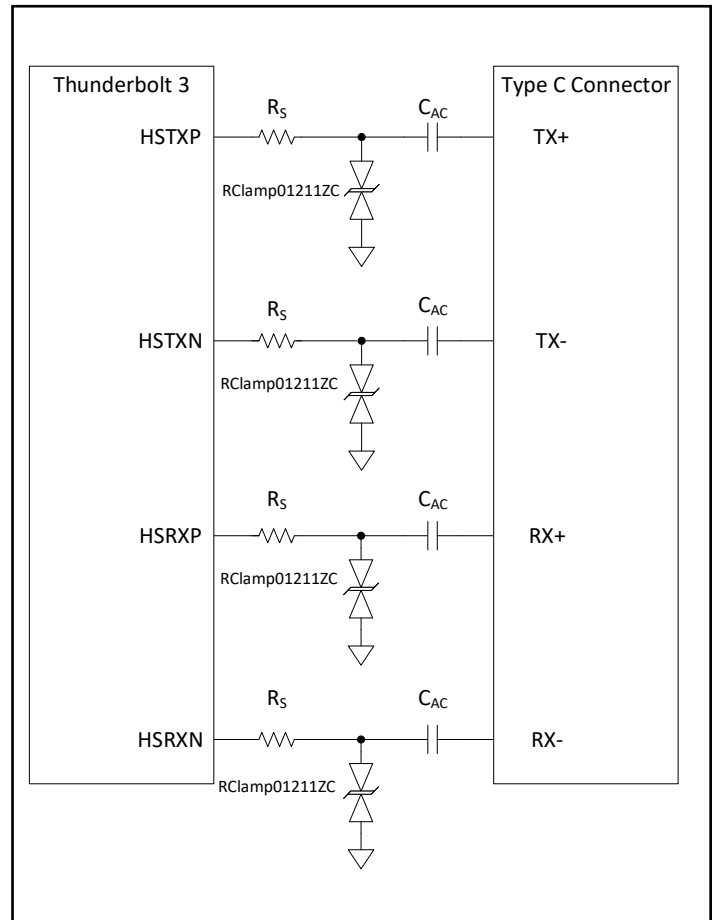
Figure 3- Thunderbolt 3 Protection
