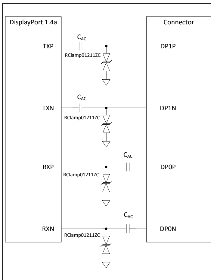
Figure 1 - DisplayPort Line Protection
