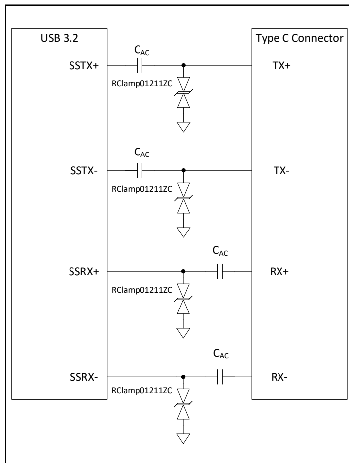
Figure 2 - USB 3.2 Protection
