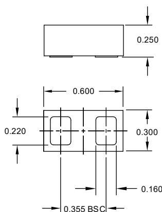
Nominal Dimensions in mm
