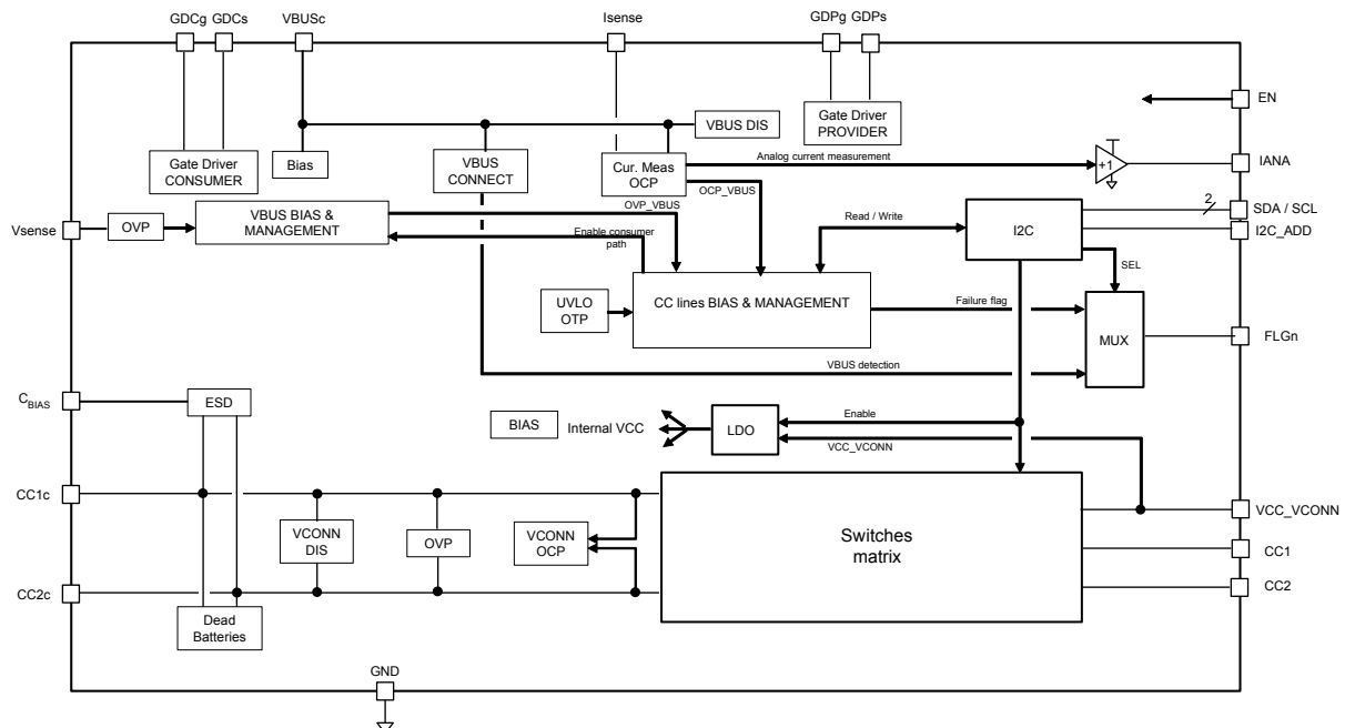
Figure 3. Internal block diagram
