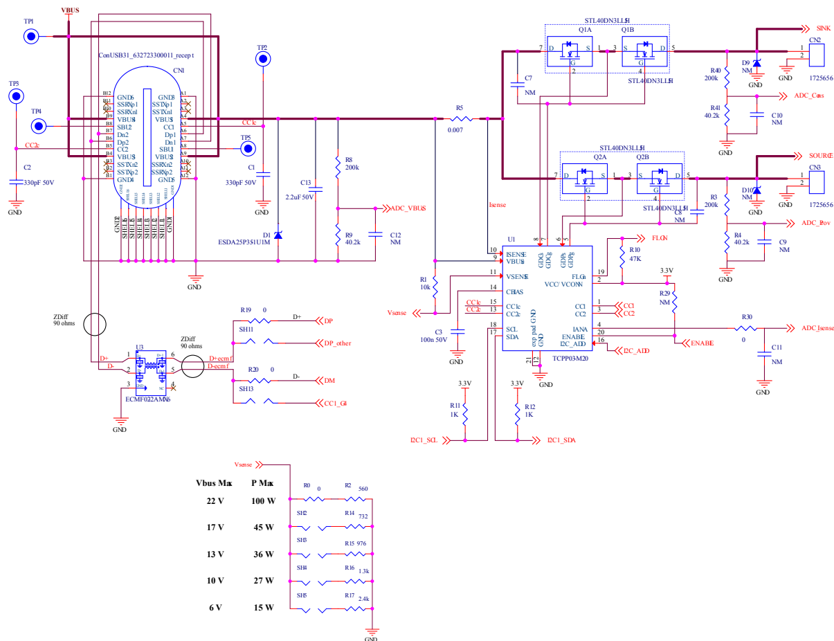
Figure 15. Schematic extract of nucleo expansion board X-NUCLEO-DRP1M1 using TCPP03-M20
