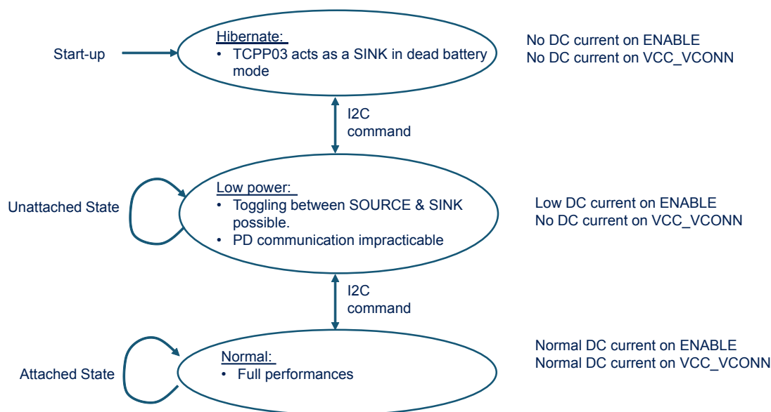
Figure 10. Power mode process
