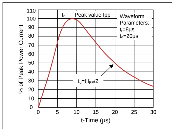
Figure 2. Pulse Waveforms
