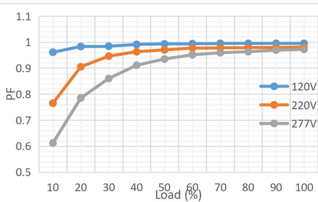
Power Factor Vs Different Loads
