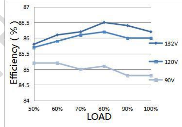
Fig.4 Efficiency-Load Curve:
