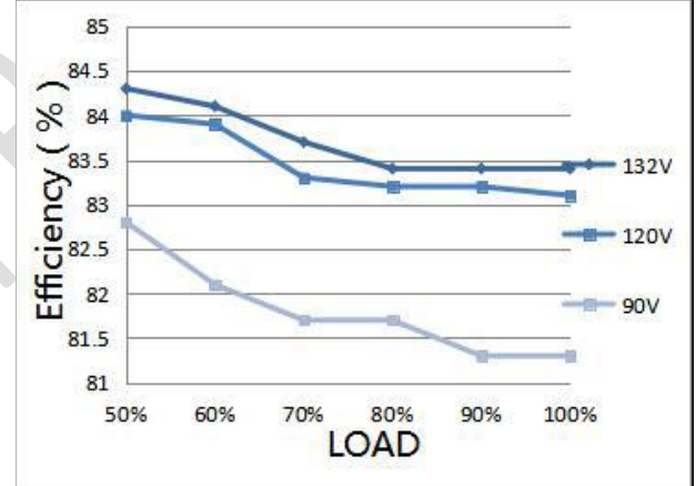
Fig.4 Efficiency-Load Curve:
