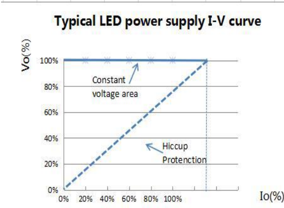
Fig.3 I-V Curve:
