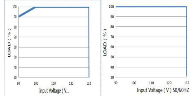
Fig.2 Static Characteristics Curve:
