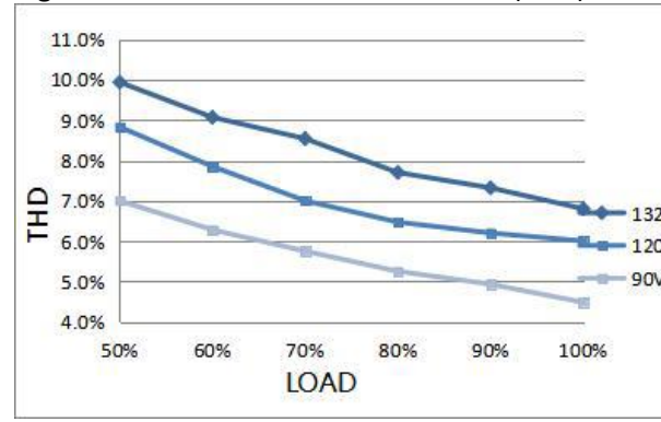
Fig.6 Total Harmonic Distortion Curve (THD):
