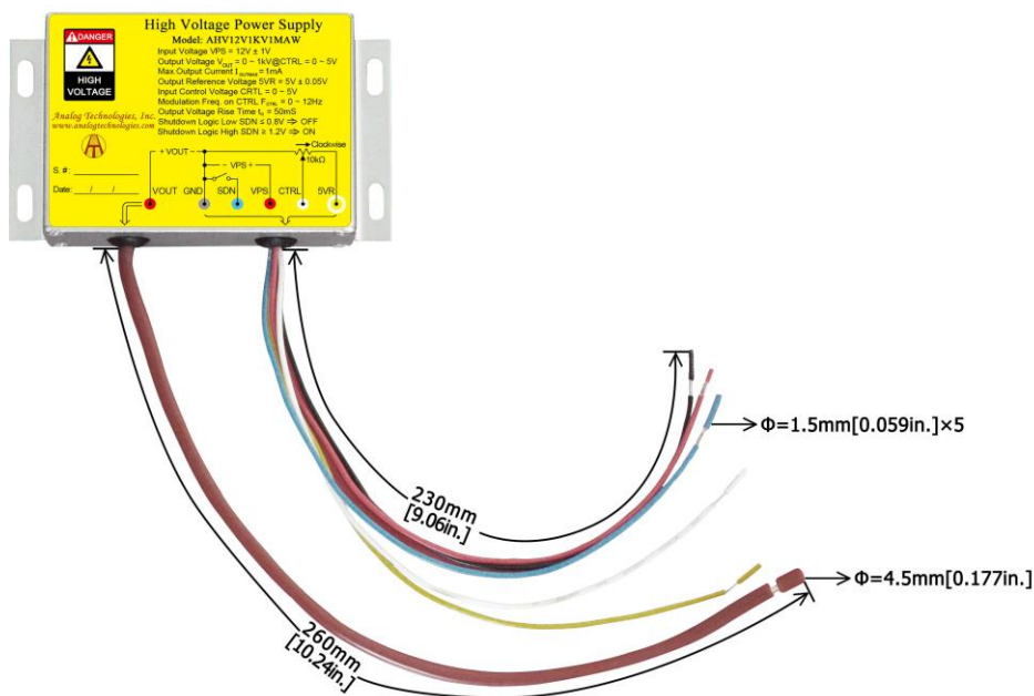
Figure 13. Connecting Lead Wires of AHV12V1KV1MAW
