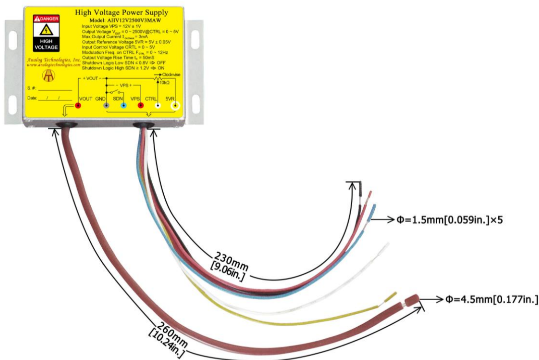
Figure 13. Connecting Lead Wires of AHV12V2500V3MAW
