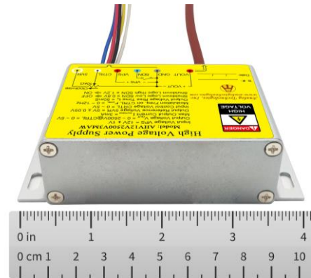
Figure 1.3. Side View
