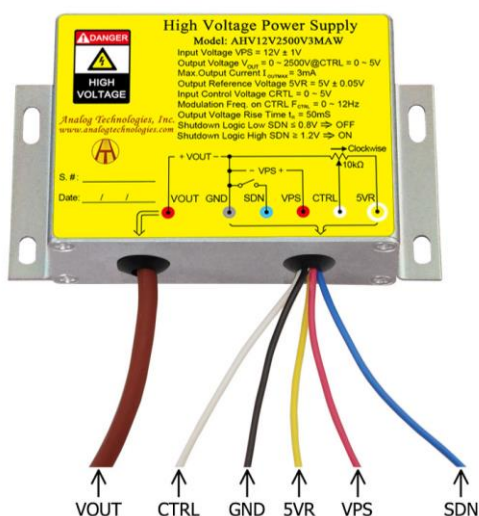
Figure 2. The Connecting Lead Wires of AHV12V2500V3MAW
