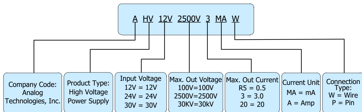
Naming Principle of AHV12V2500V3MAW
