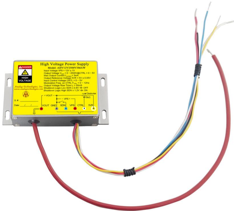
Figure 1.1. Top View of AHV12V2500V3MAW
