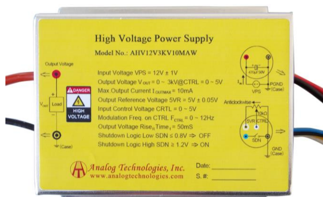
Figure 1. Physical Photo of AHV12V3KV10MAW
