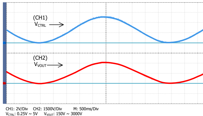
Figure 8. Sine Wave Modulation
