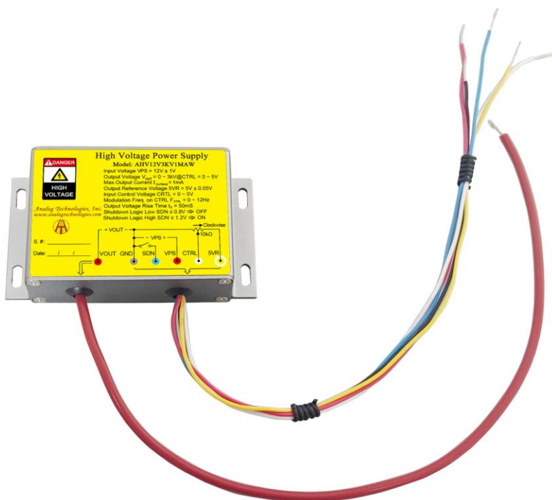
Figure 1.1. Top View of AHV12V3KV1MAW
