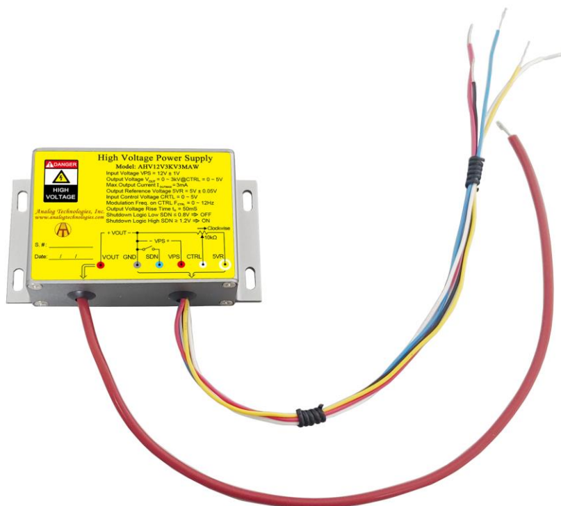
Figure 1.1. Top View of AHV12V3KV3MAW
