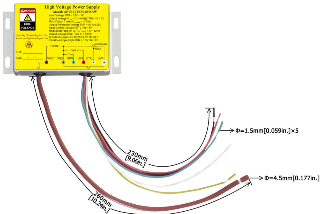
Figure 13. Connecting Lead Wires of AHV12V4KV2R5MAW
