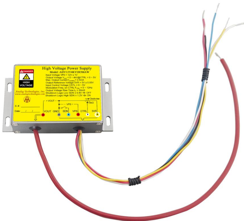
Figure 1.1. Top View of AHV12V4KV2R5MAW
