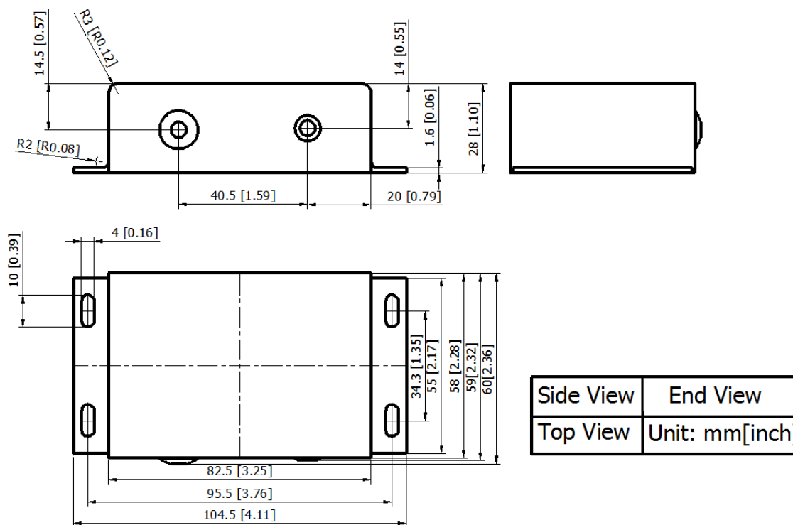
Figure 14. Outline Dimensions
