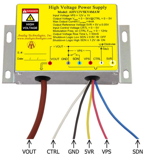
Figure 2. The Connecting Lead Wires of AHV12V5KV4MAW
