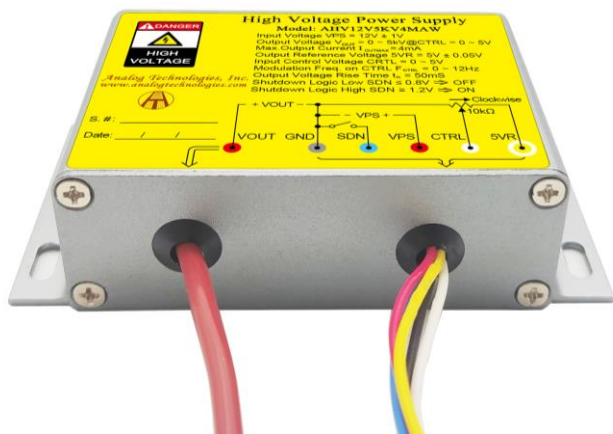
Figure 1.2. Side View
