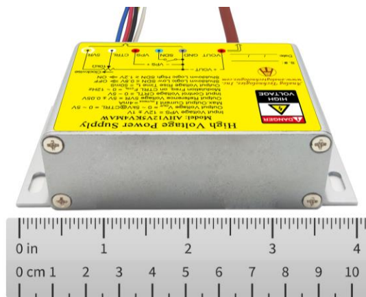
Figure 1.3. Side View
