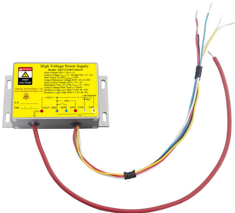
Figure 1.1. Top View of AHV12V6KV1MAW
