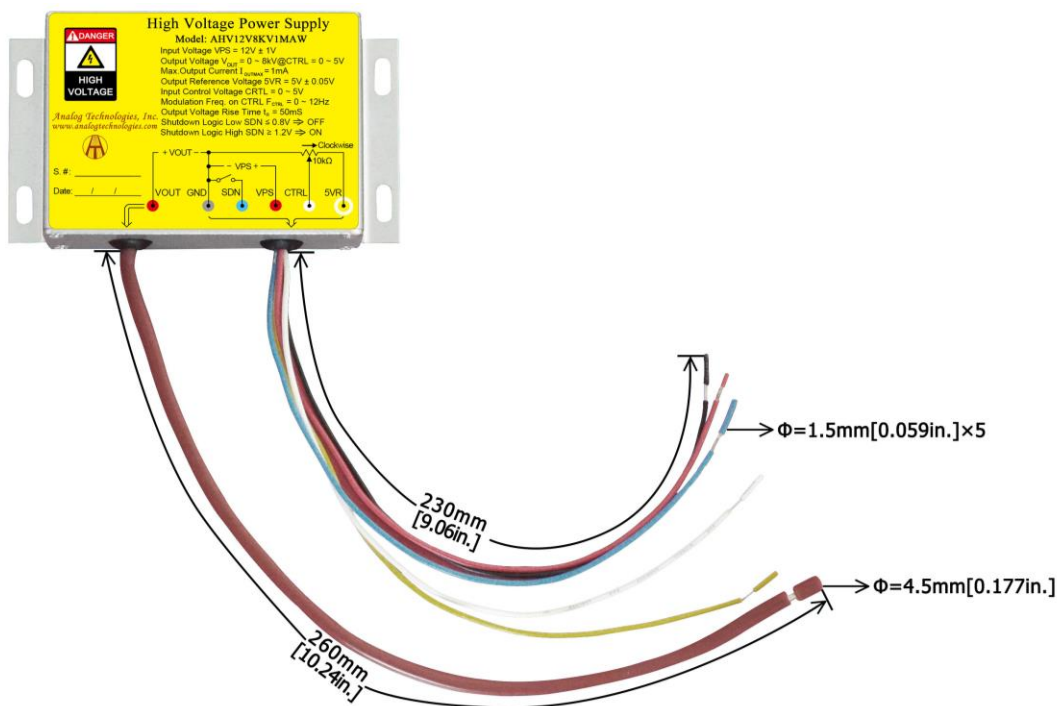
Figure 13. Connecting Lead Wires of AHV12V8KV1MAW
