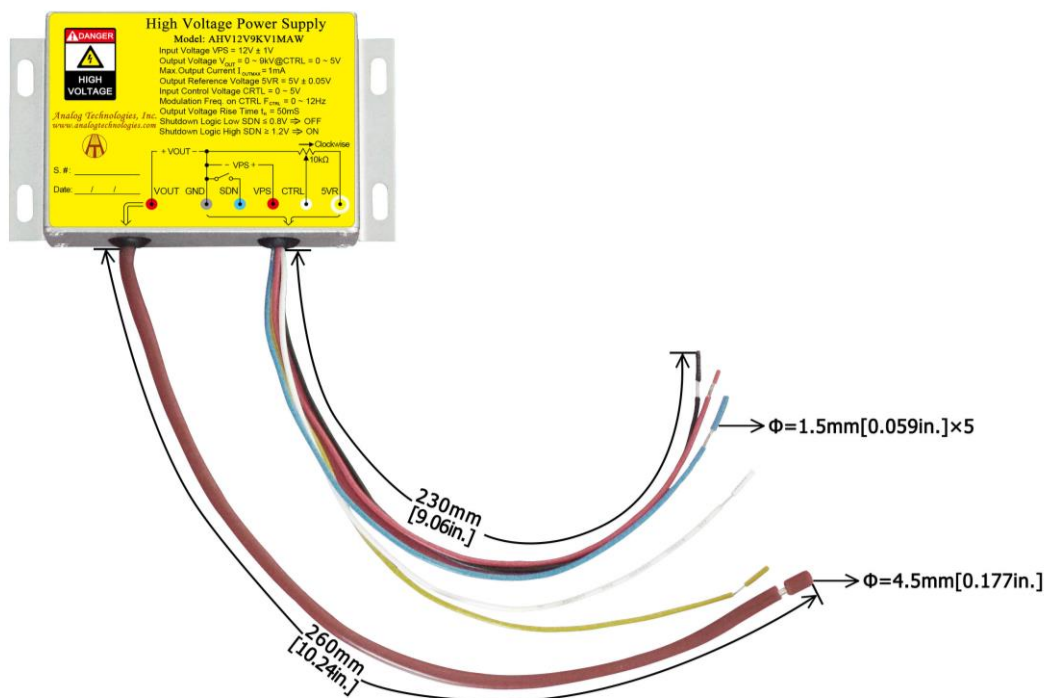
Figure 13. Connecting Lead Wires of AHV12V9KV1MAW
