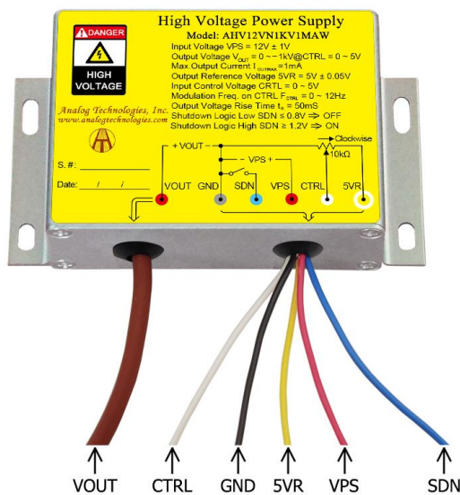
Figure 2. The Connecting Lead Wires of AHV12VN1KV1MAW
