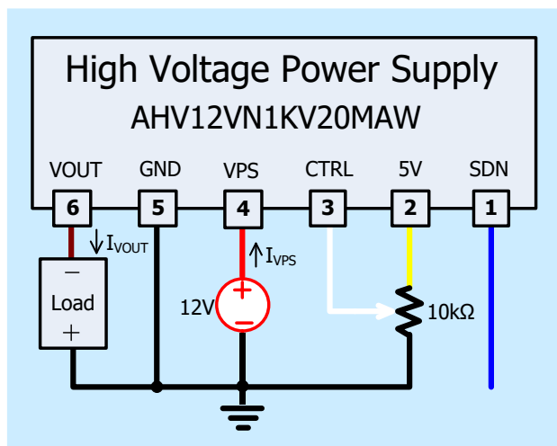
Figure 3. Setting Output to be a Constant Voltage
