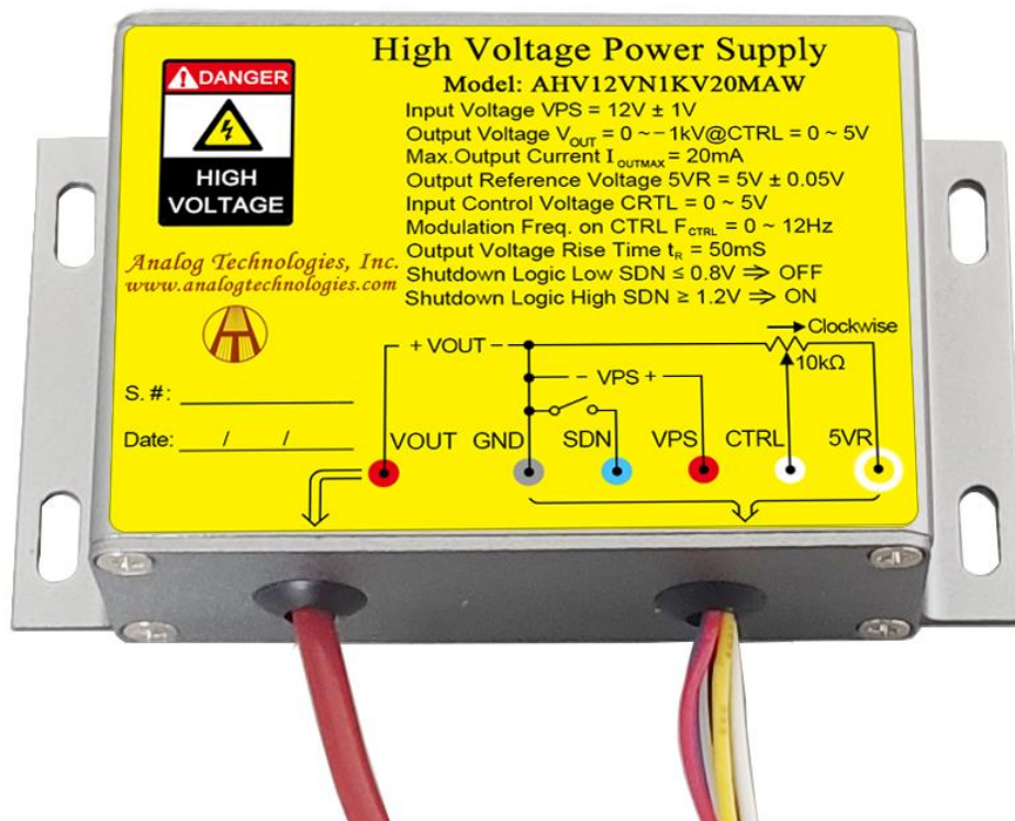
Figure 1.1. Top View of AHV12VN1KV20MAW
