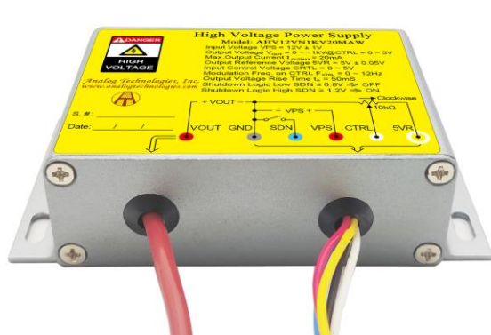
Figure 1.2. Side View
