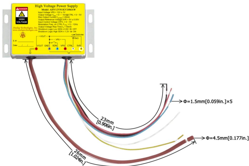
Figure 13. Connecting Lead Wires of AHV12VN1KV20MAW
