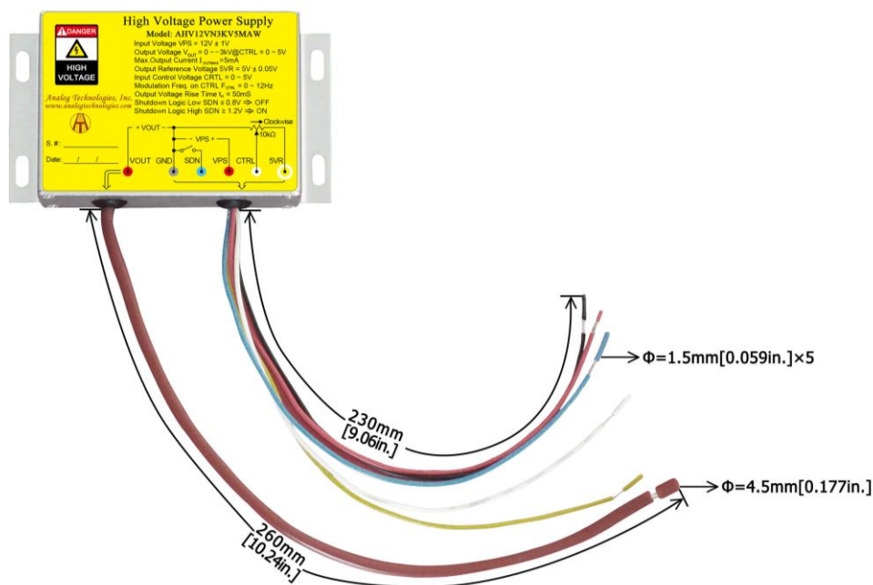
Figure 13. Connecting Lead Wires of AHV12VN3KV5MAW
