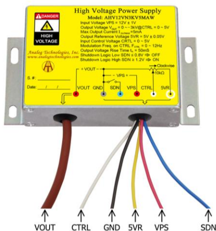
Figure 2. The Connecting Lead Wires of AHV12VN3KV5MAW
