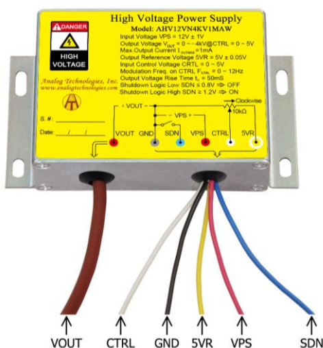
Figure 2. The Connecting Lead Wires of AHV12VN4KV1MAW
