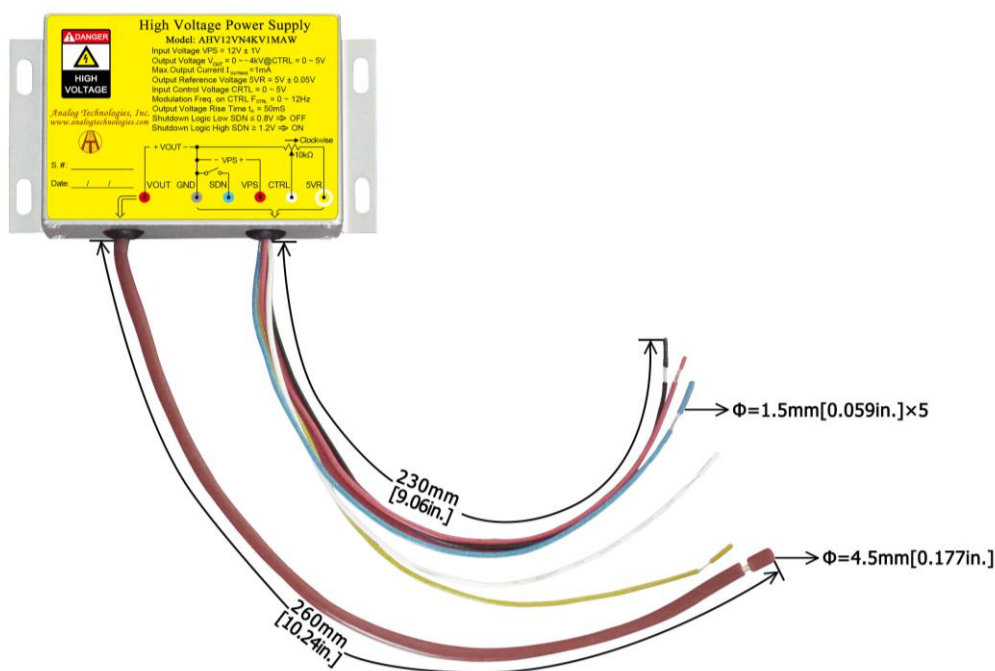
Figure 13. Connecting Lead Wires of AHV12VN4KV1MAW
