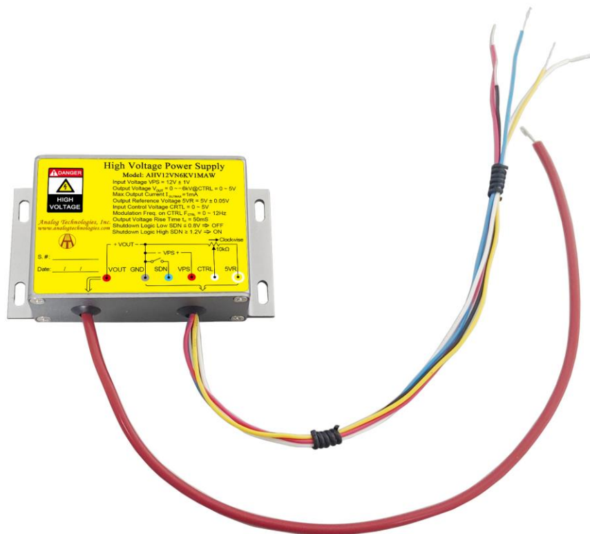
Figure 1.1. Top View of AHV12VN6KV1MAW
