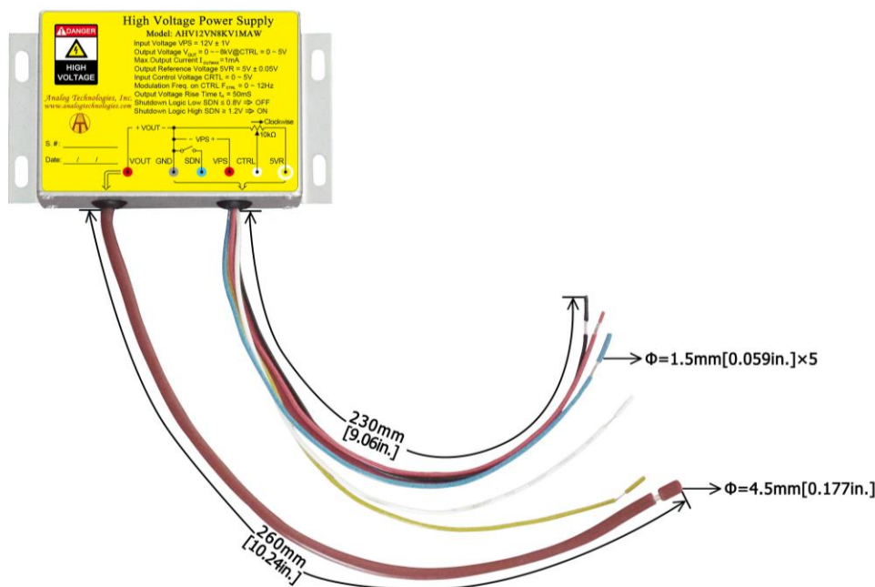
Figure 13. Connecting Lead Wires of AHV12VN8KV1MAW
