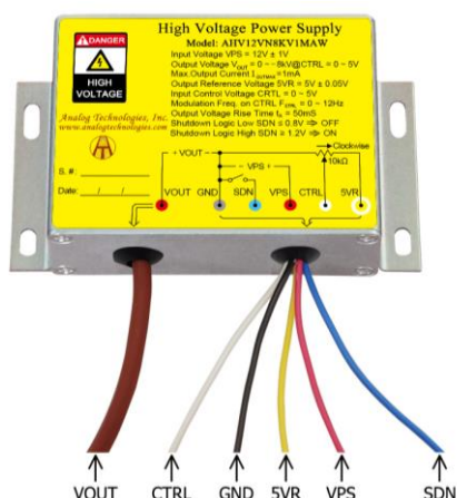
Figure 2. The Connecting Lead Wires of AHV12VN8KV1MAW
