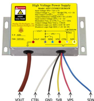
Figure 2. The Connecting Lead Wires of AHV12VN8KV2R5MAW
