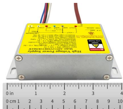
Figure 1.1. Top View of AHV12VN8KV2R5MAW
