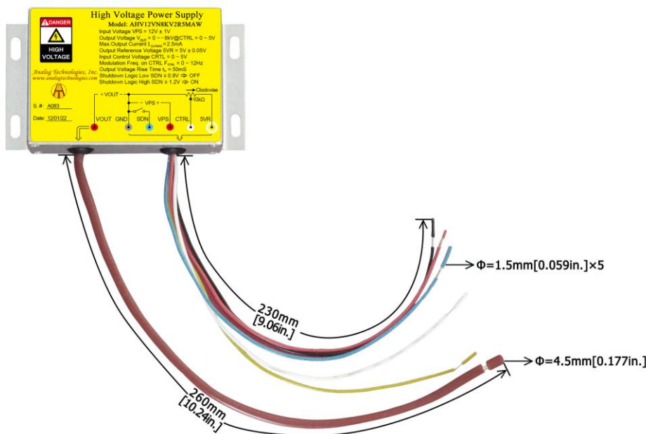
Figure 13. Connecting Lead Wires of AHV12VN8KV2R5MAW
