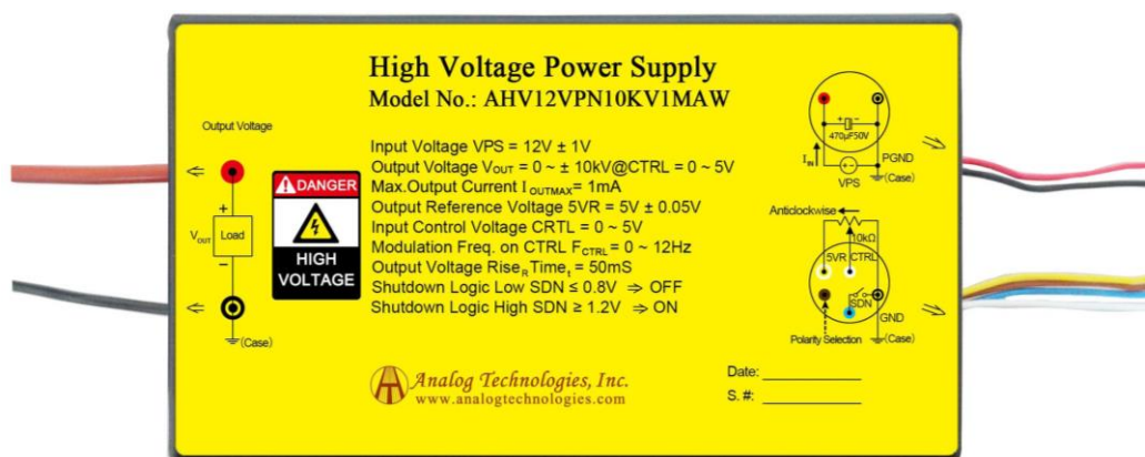
Figure 1. Top View of AHV12VPN10KV1MAW
