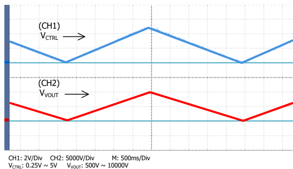
Figure 6A. Triangle Wave Modulation ( V_{OUT}=10kV )
