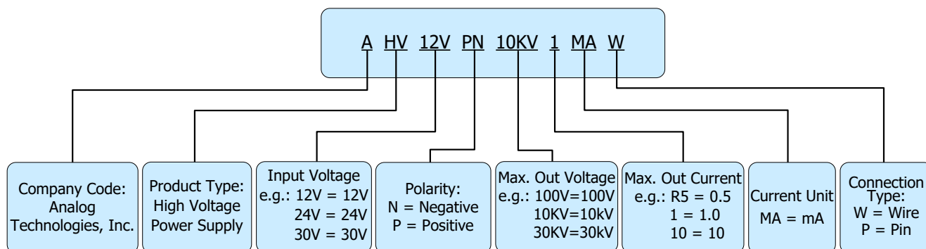
Figure 11. Naming Principle of AHV12VPN10KV1MAW
