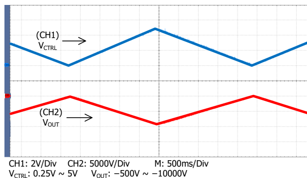
Figure 6B. Triangle Wave Modulation ( V_{OUT}= -10kV )
