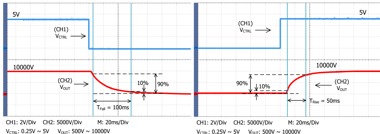
Figure 9A. Falling Trail for Large Signal Response
