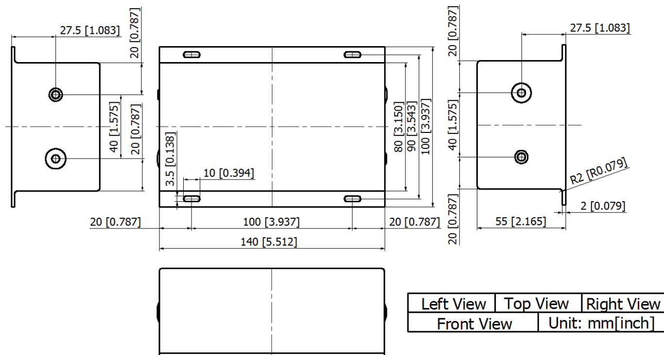
Figure 13. Outline Dimensions
