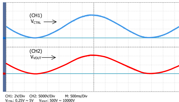
Figure 7A. Sine Wave Modulation ( V_{OUT}=10kV )
