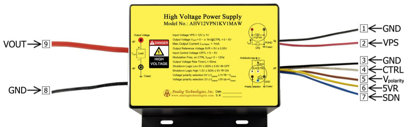
Figure 2. The Connecting Lead Wires of AHV12VPN10KV1MAW
