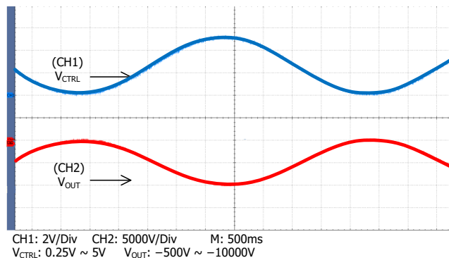
Figure 7B. Sine Wave Modulation ( V_{OUT}= -10kV )
