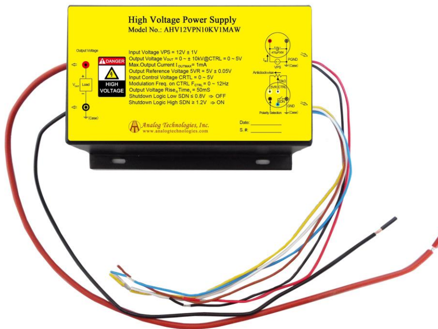
Figure 12. Connecting Lead Wires of AHV12VPN10KV1MAW
