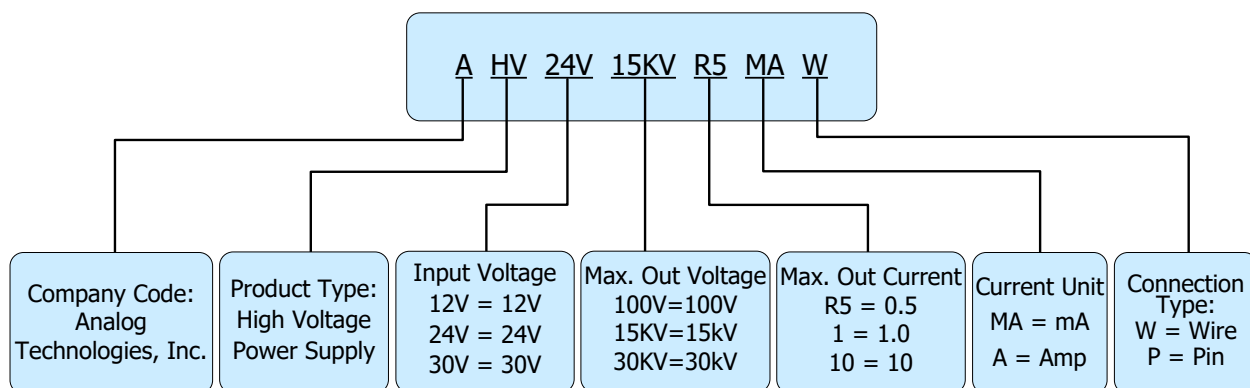
Naming Principle of AHV24V15KVR5MAW
