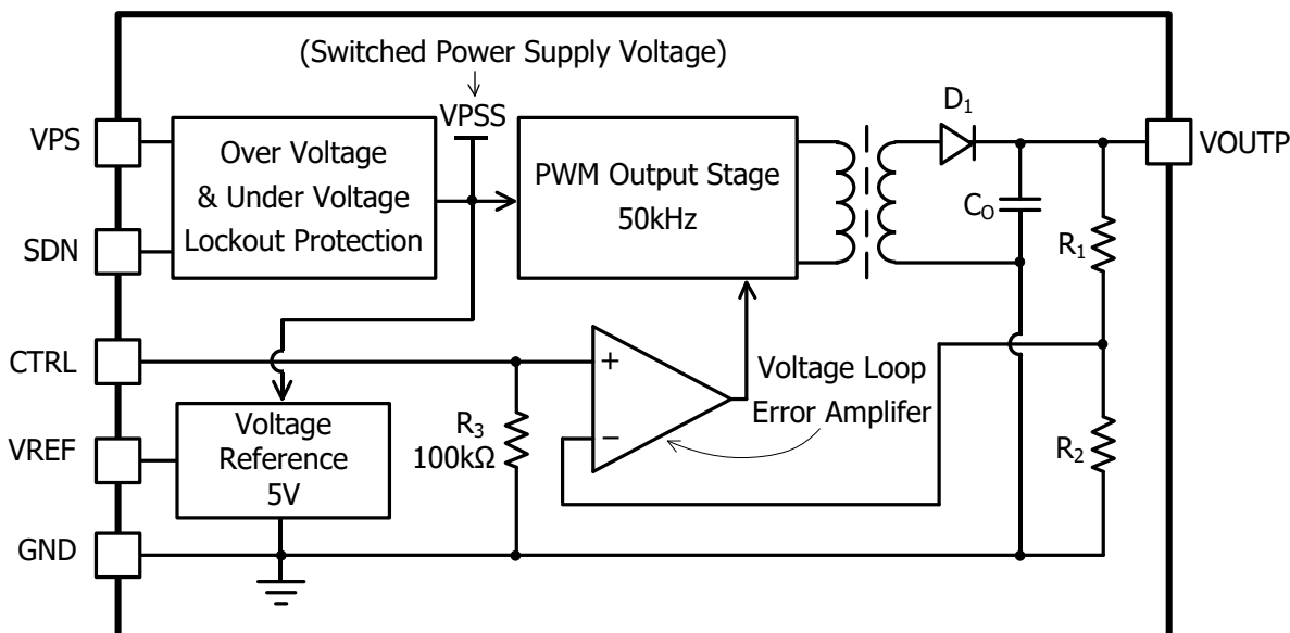
Figure 6. High Voltage Power Supply Function Block Diagram
