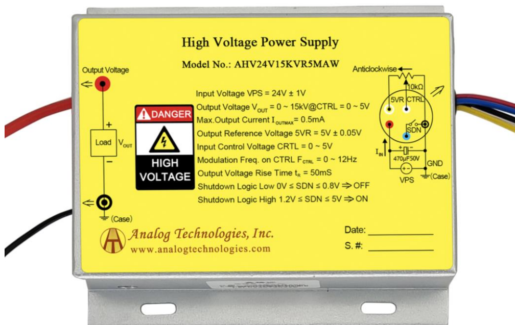
Figure 1.1. Top View of AHV24V15KVR5MAW
