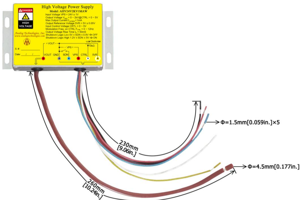
Figure 13. Connecting Lead Wires of AHV24V2KV1MAW
