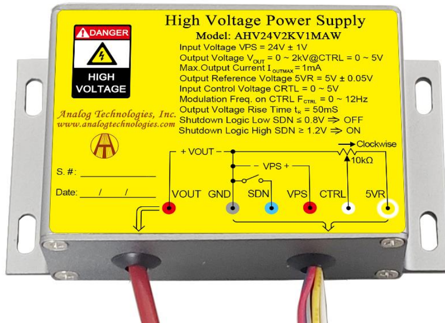
Figure 1.1. Top View of AHV24V2KV1MAW
