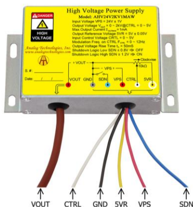
Figure 2. The Connecting Lead Wires of AHV24V2KV1MAW
