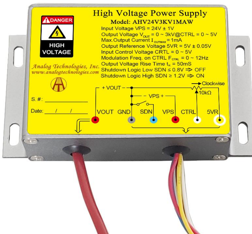
Figure 1.1. Top View of AHV24V3KV1MAW
