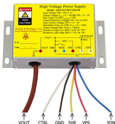
Figure 2. The Connecting Lead Wires of AHV24V3KV1MAW
