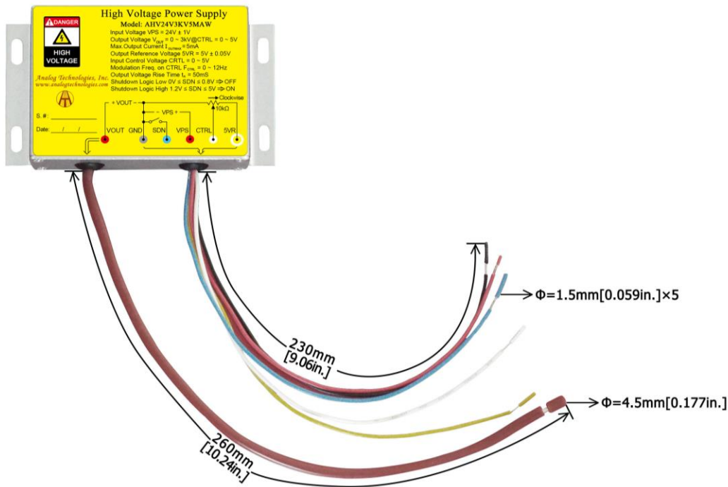
Figure 13. Connecting Lead Wires of AHV24V3KV5MAW
