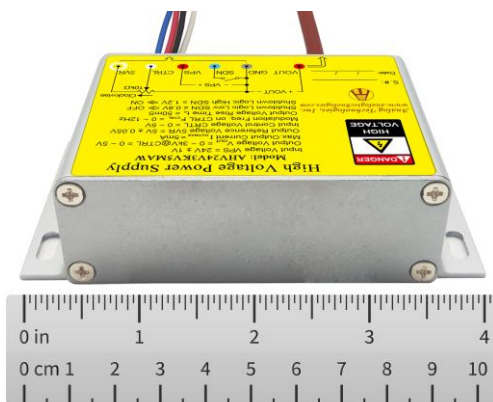
Figure 1.3. Side View
