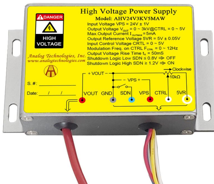
Figure 1.1. Top View of AHV24V3KV5MAW
