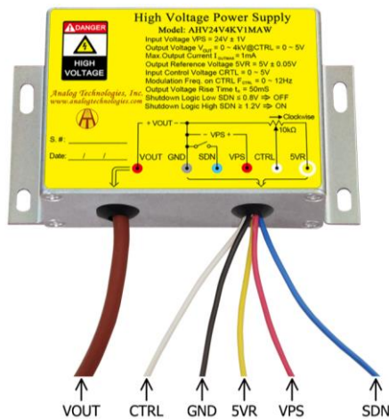
Figure 2. The Connecting Lead Wires of AHV24V4KV1MAW
