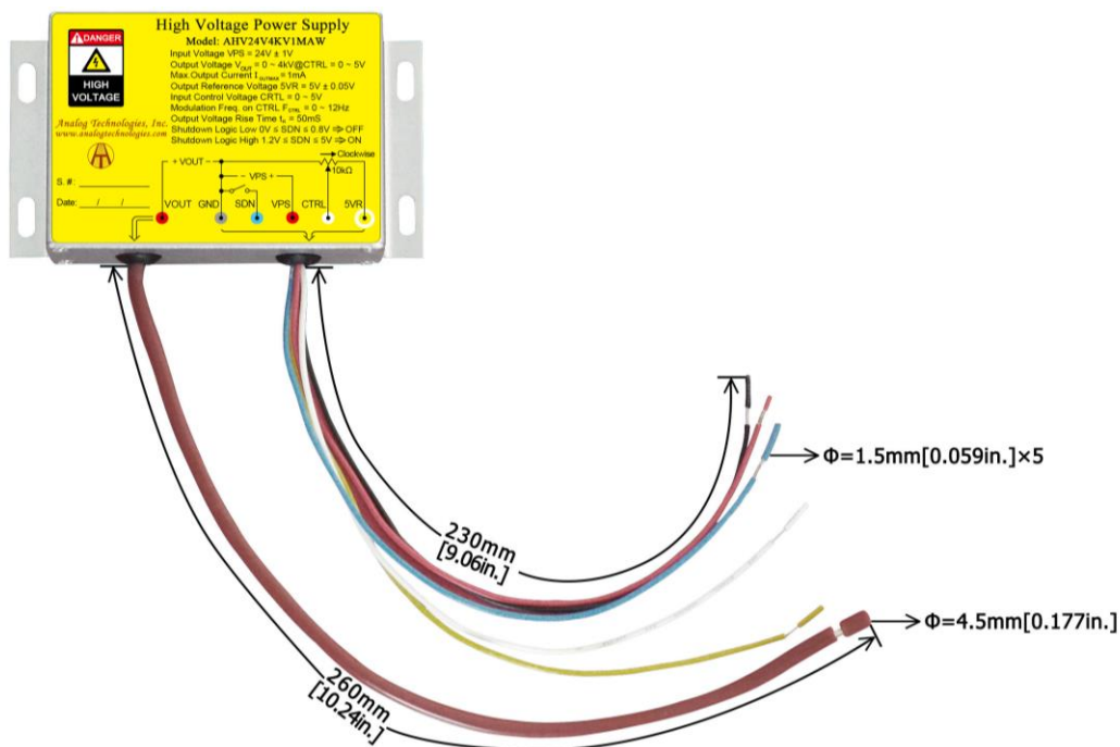
Figure 13. Connecting Lead Wires of AHV24V4KV1MAW
