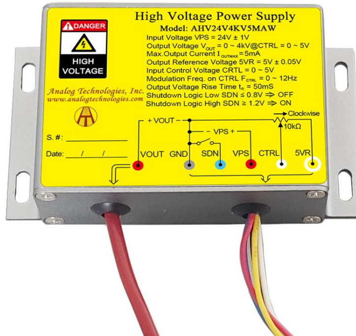
Figure 1.1. Top View of AHV24V4KV5MAW
