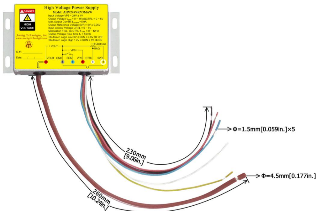
Figure 13. Connecting Lead Wires of AHV24V4KV5MAW
