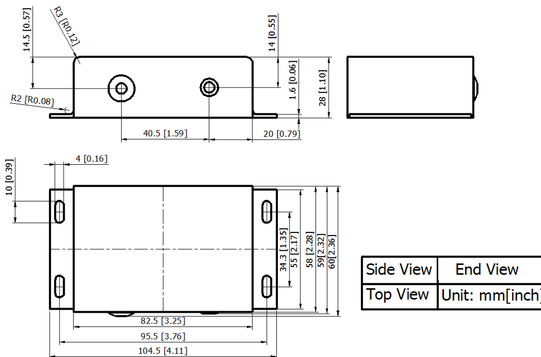
Figure 14. Outline Dimensions
