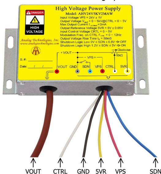
Figure 2. The Connecting Lead Wires of AHV24V5KV2MAW
