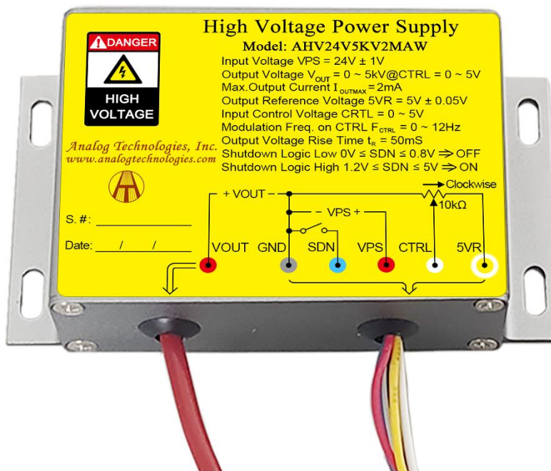
Figure 1.1. Top View of AHV24V5KV2MAW
