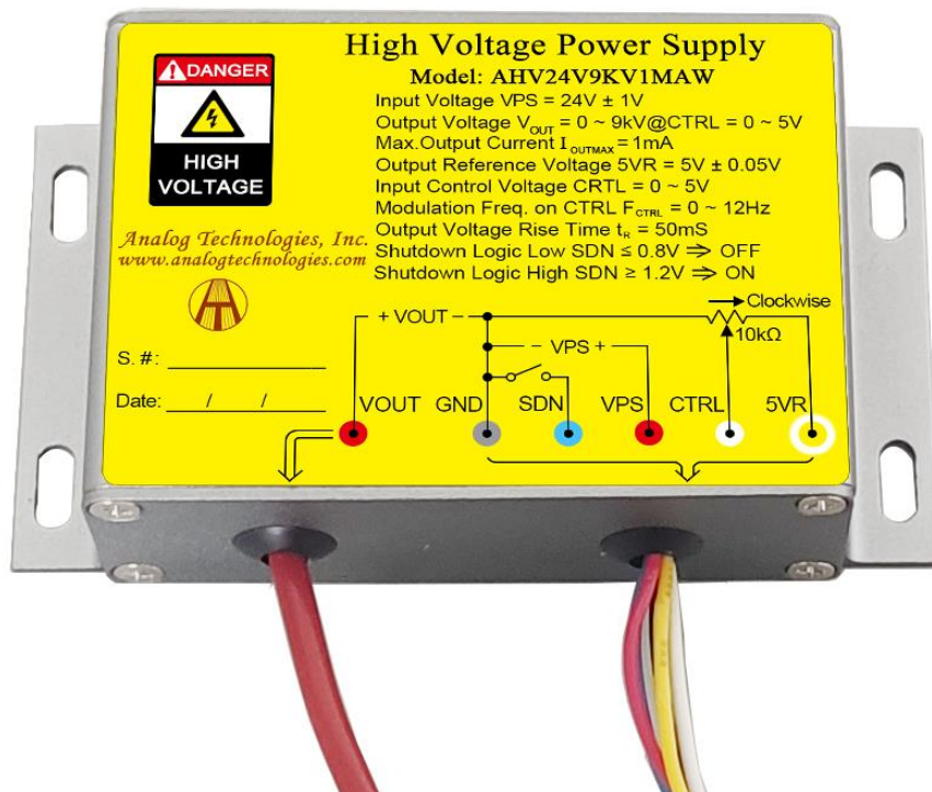
Figure 1.1. Top View of AHV24V9KV1MAW
