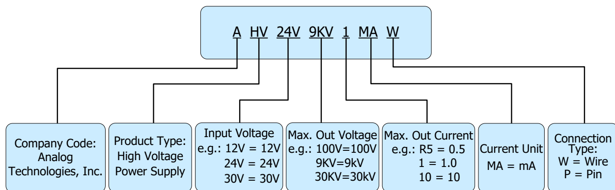
Naming Principle of AHV24V9KV1MAW
