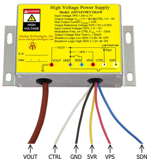
Figure 2. The Connecting Lead Wires of AHV24V9KV1MAW
