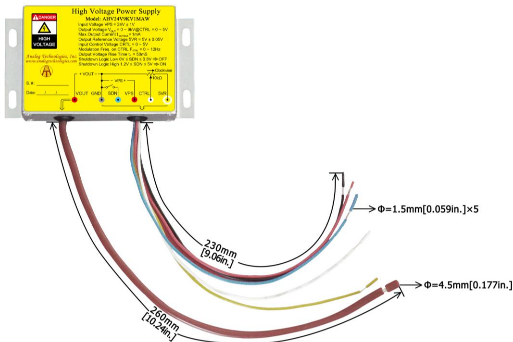
Figure 13. Connecting Lead Wires of AHV24V9KV1MAW
