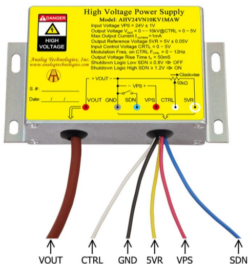
Figure 2. The Connecting Lead Wires of AHV24VN10KV1MAW
