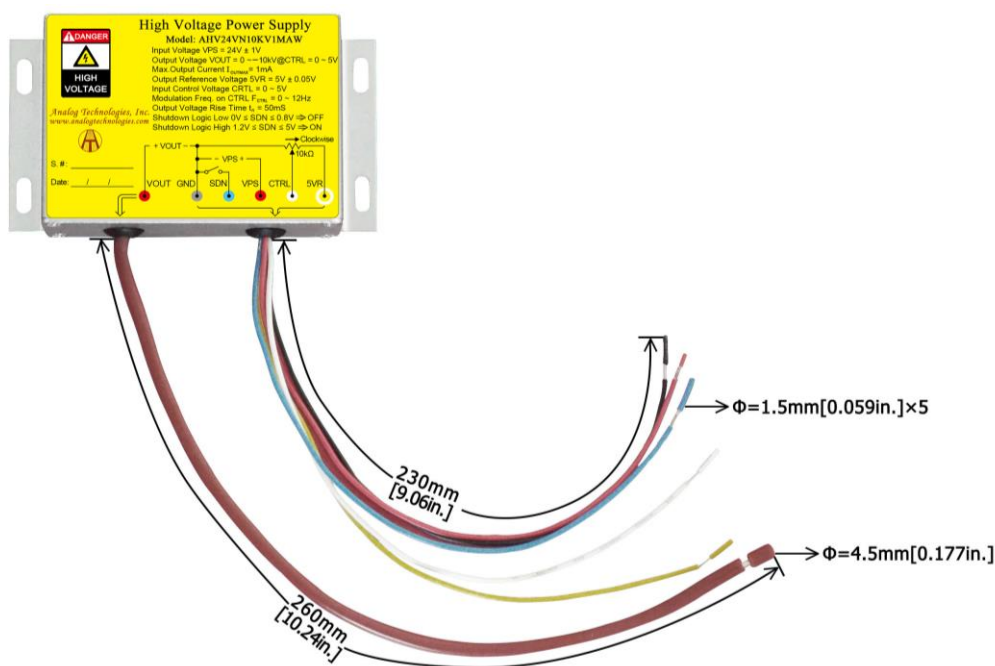
Figure 13. Connecting Lead Wires of AHV24VN10KV1MAW
