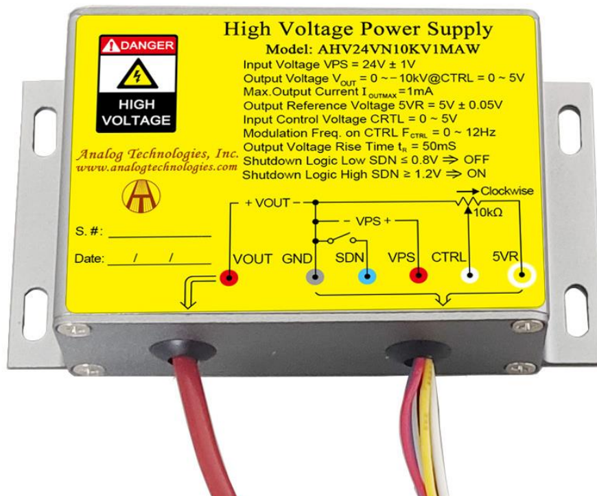
Figure 1.1. Top View of AHV24VN10KV1MAW
