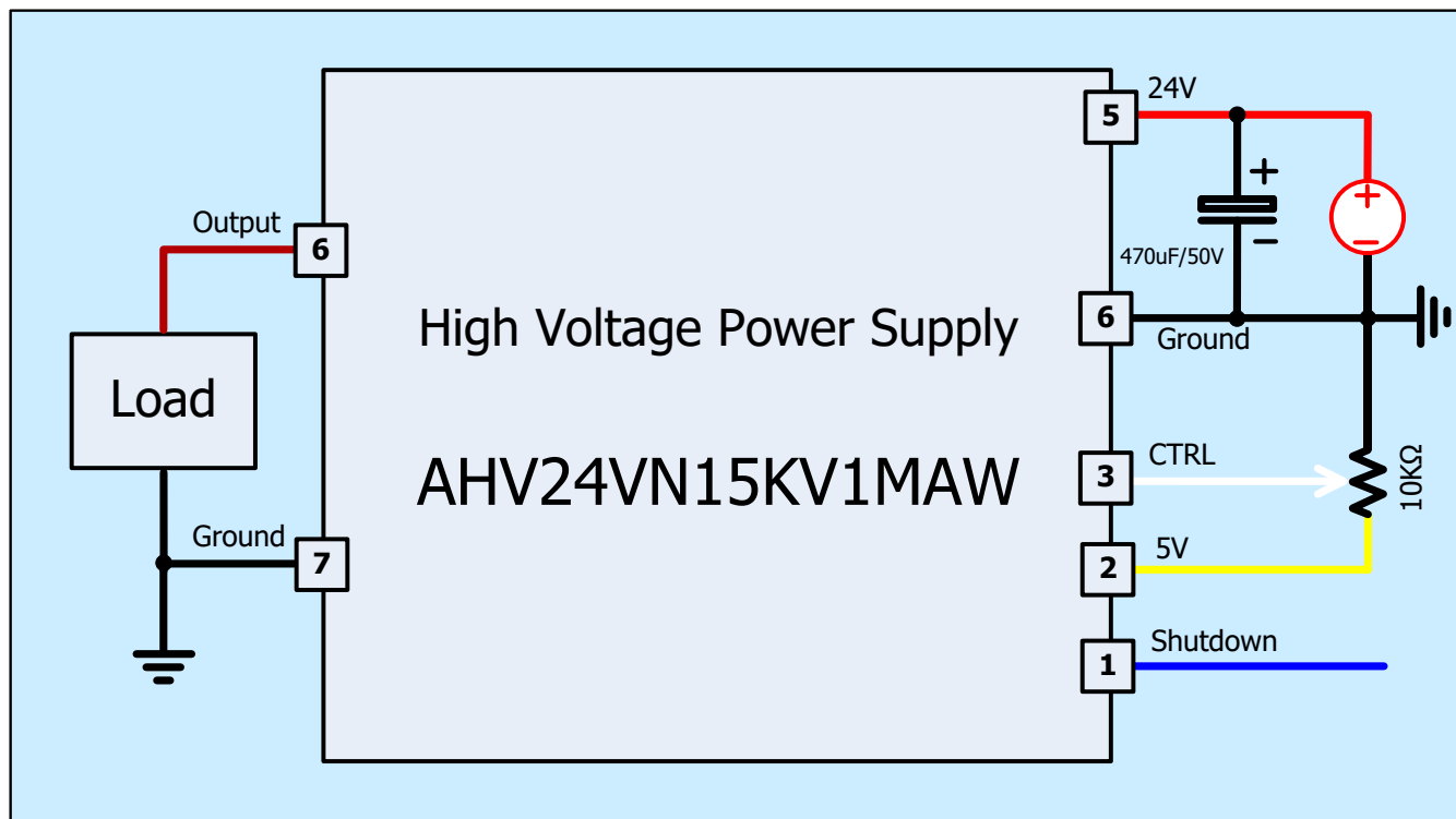
Figure 3. Setting Output to be a Constant Voltage
