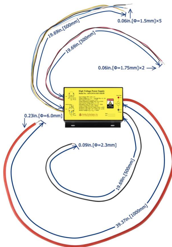
Figure 13. Connecting Lead Wires of AHV24VN15KV1MAW
