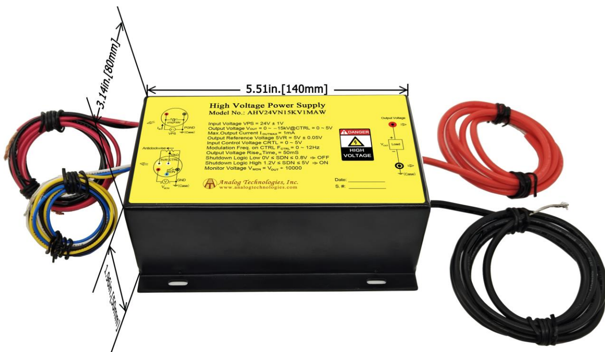
Figure 1.1. Top View of AHV24VN15KV1MAW
