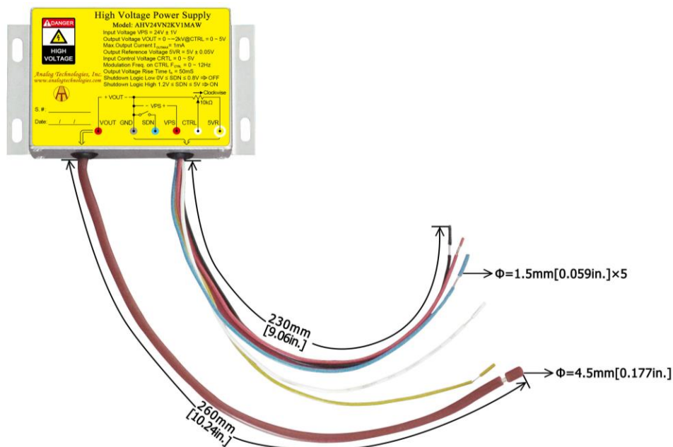
Figure 13. Connecting Lead Wires of AHV24VN2KV1MAW
