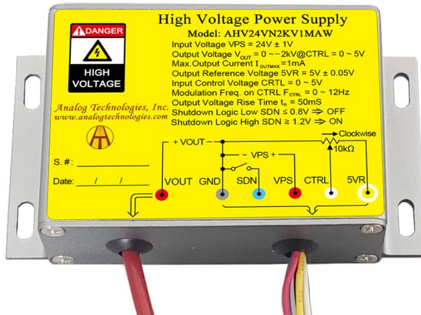
Figure 1.1. Top View of AHV24VN2KV1MAW
