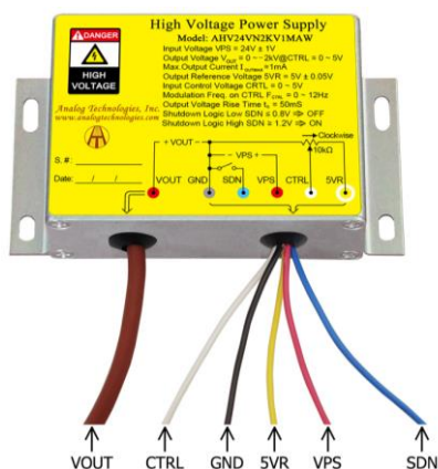
Figure 2. The Connecting Lead Wires of AHV24VN2KV1MAW
