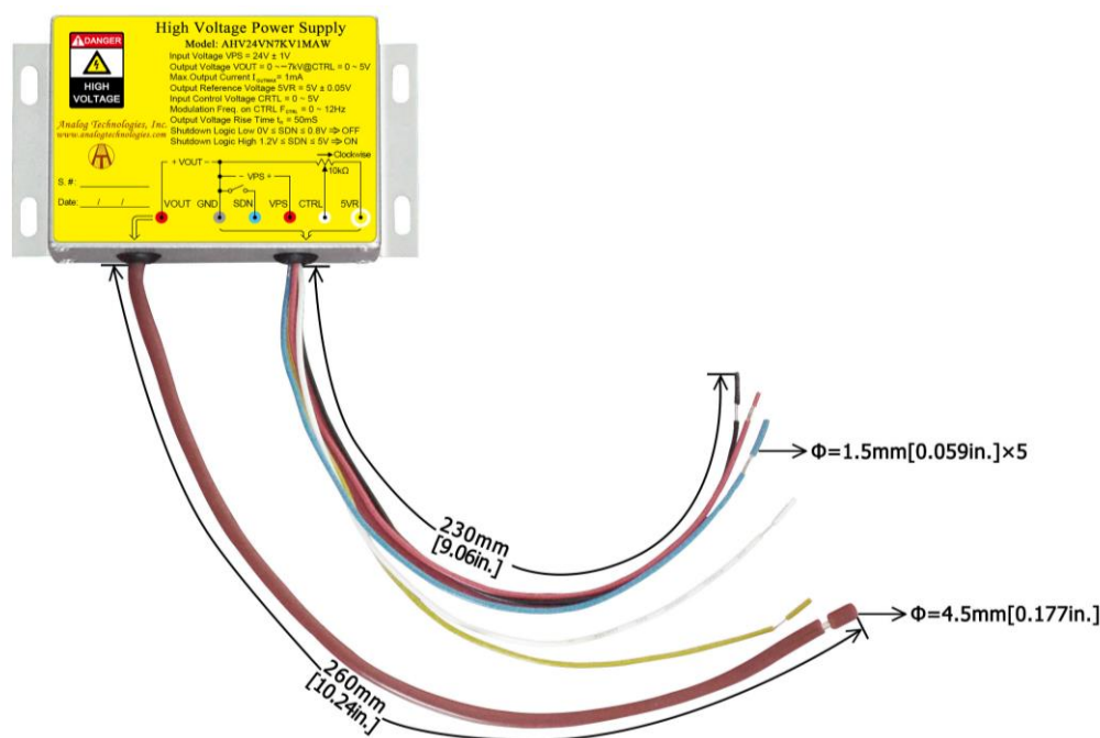
Figure 13. Connecting Lead Wires of AHV24VN7KV1MAW
