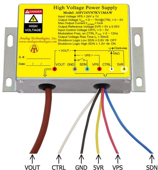
Figure 2. The Connecting Lead Wires of AHV24VN7KV1MAW
