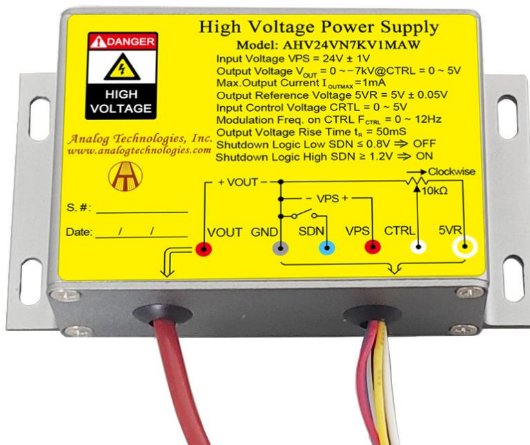
Figure 1.1. Top View of AHV24VN7KV1MAW
