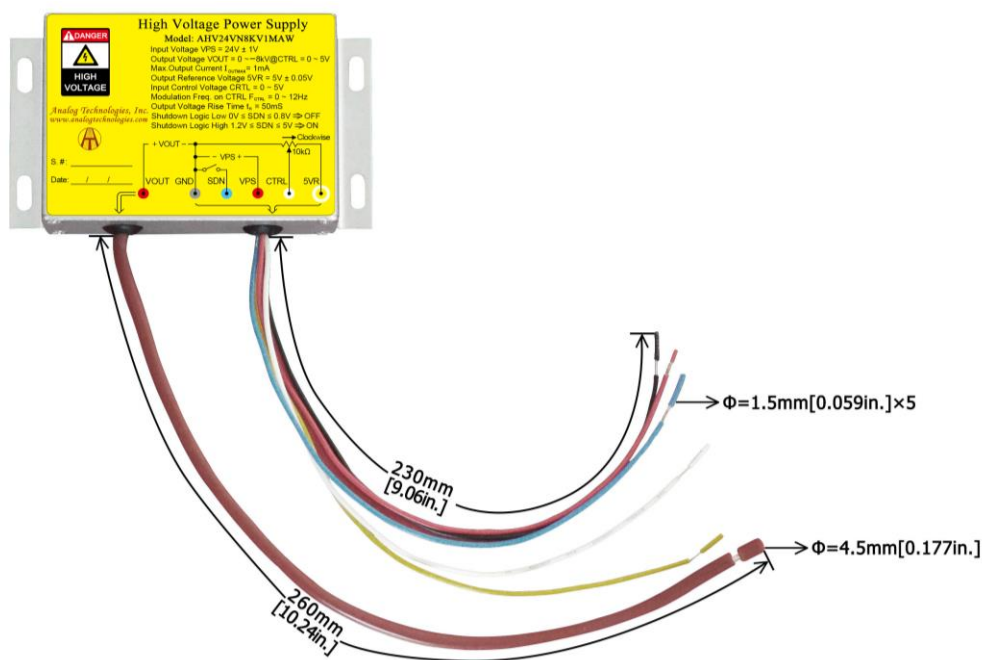
Figure 13. Connecting Lead Wires of AHV24VN8KV1MAW
