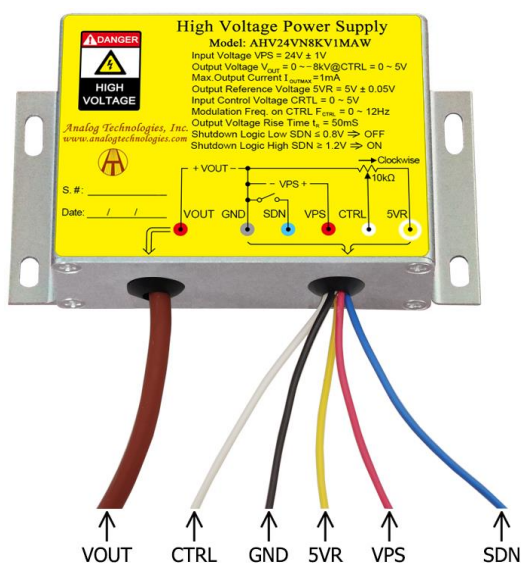
Figure 2. The Connecting Lead Wires of AHV24VN8KV1MAW
