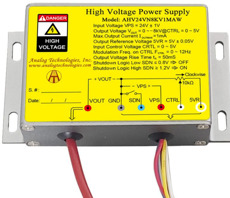
Figure 1.1. Top View of AHV24VN8KV1MAW
