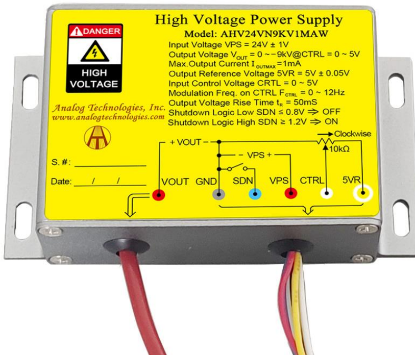
Figure 1.1. Top View of AHV24VN9KV1MAW
