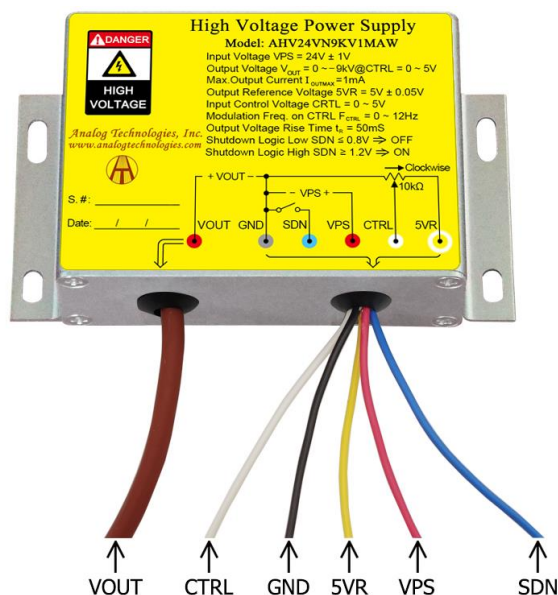
Figure 2. The Connecting Lead Wires of AHV24VN9KV1MAW
