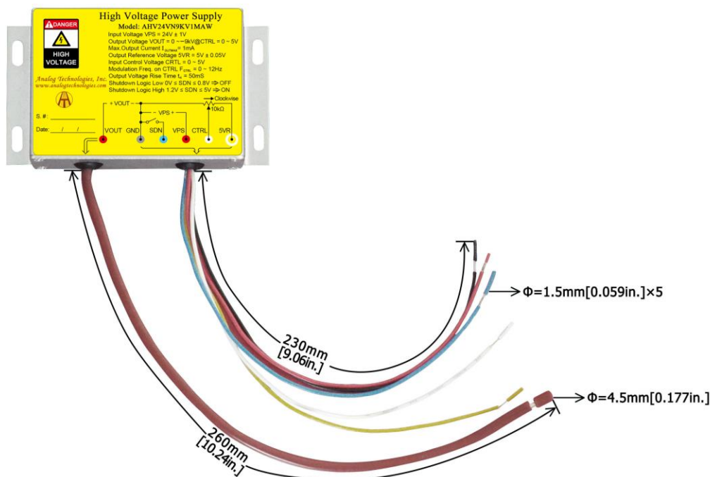
Figure 13. Connecting Lead Wires of AHV24VN9KV1MAW
