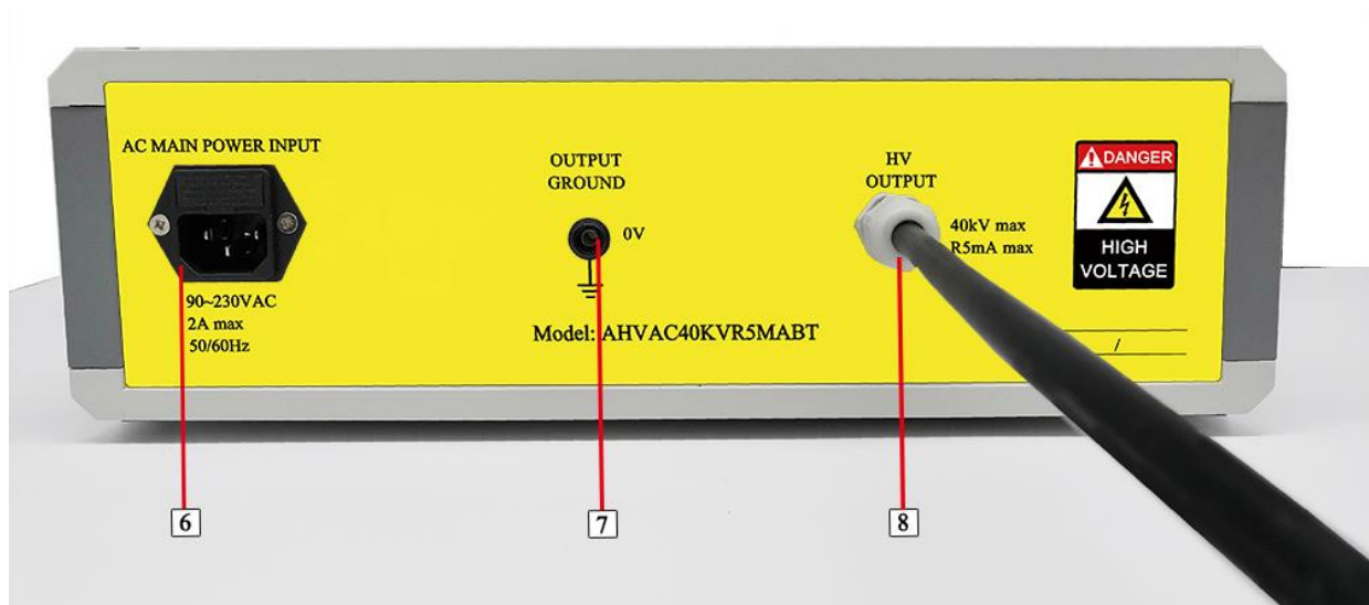
Figure 3. Back Panel
