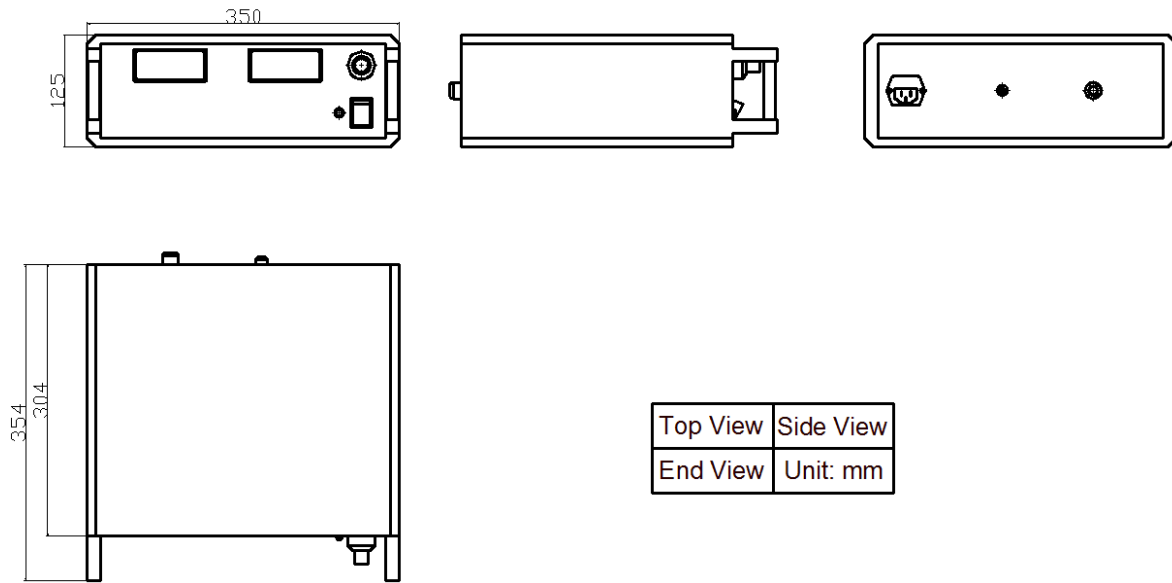
Figure 7. Dimensions for AHVAC40KVR5MABT
