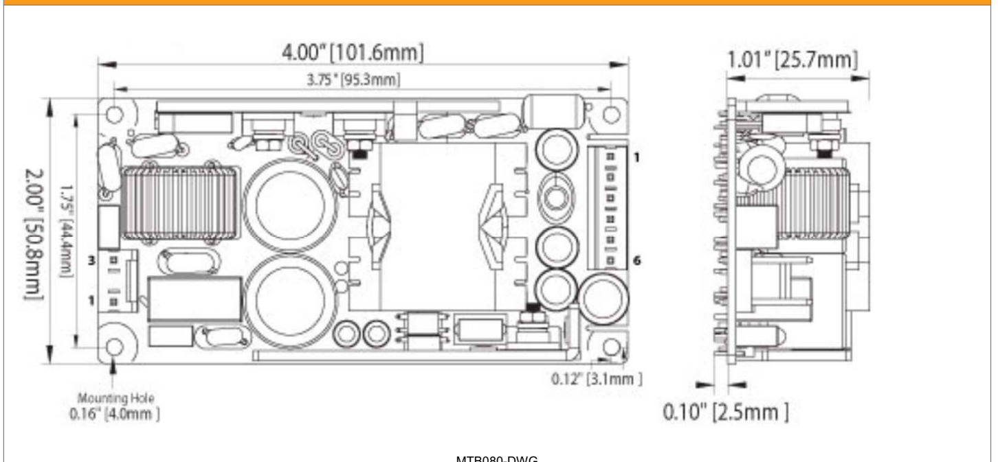
MTB080-DWG
